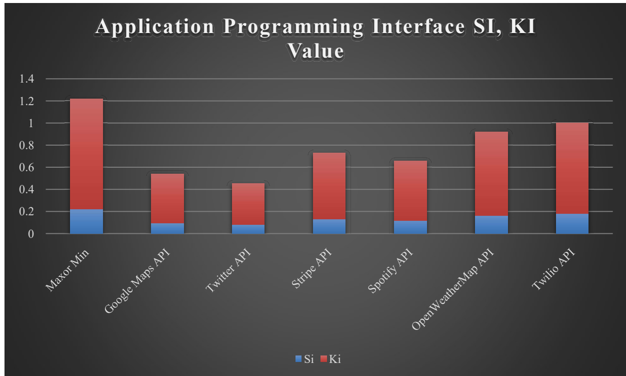
Figure 4. Application Programming Interface SI,KI Value
